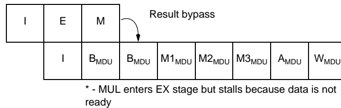
Figure 2.8 Multiply With Dependency From Load Hit
