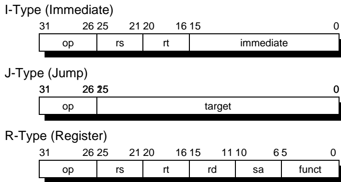
Figure 11.1 Instruction Formats
